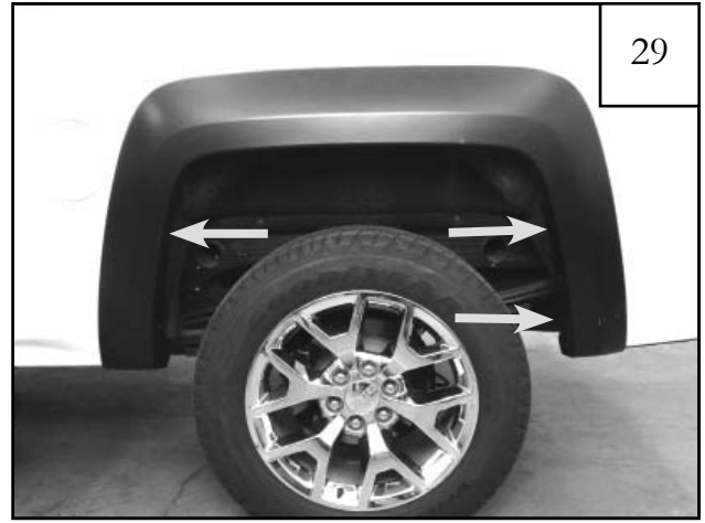
Hole locations to be marked for drilling.
